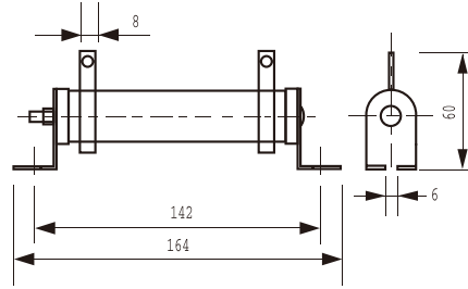
DDR50W50Ω J (50/50)
